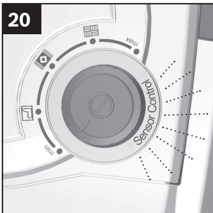
Figure 20 The display (blue ring) flashes red when the motor protection filter needs to be cleaned. The appliance is automatically adjusted to the lowest power setting.
